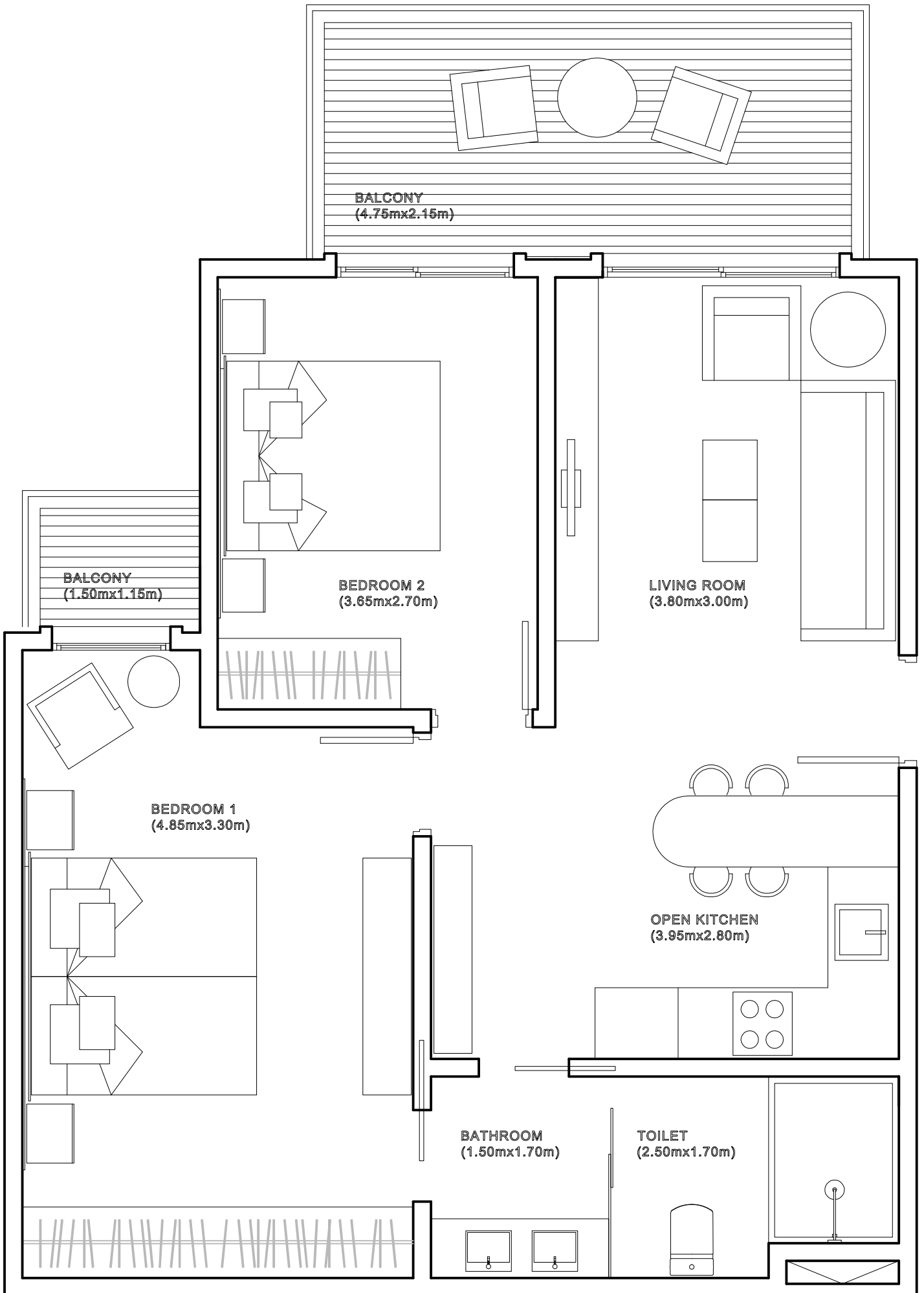
2 BEDROOM APARTMENT BUILT AREA=61 m2
